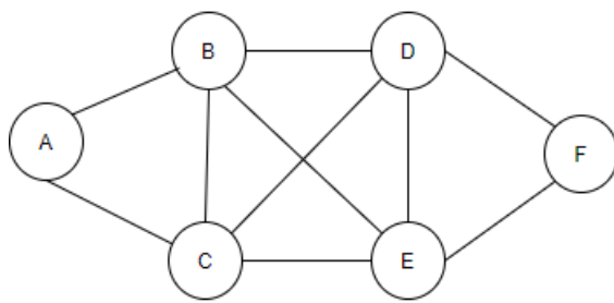
UnWeighted Graph
