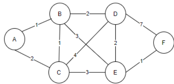
Weighted Graph
